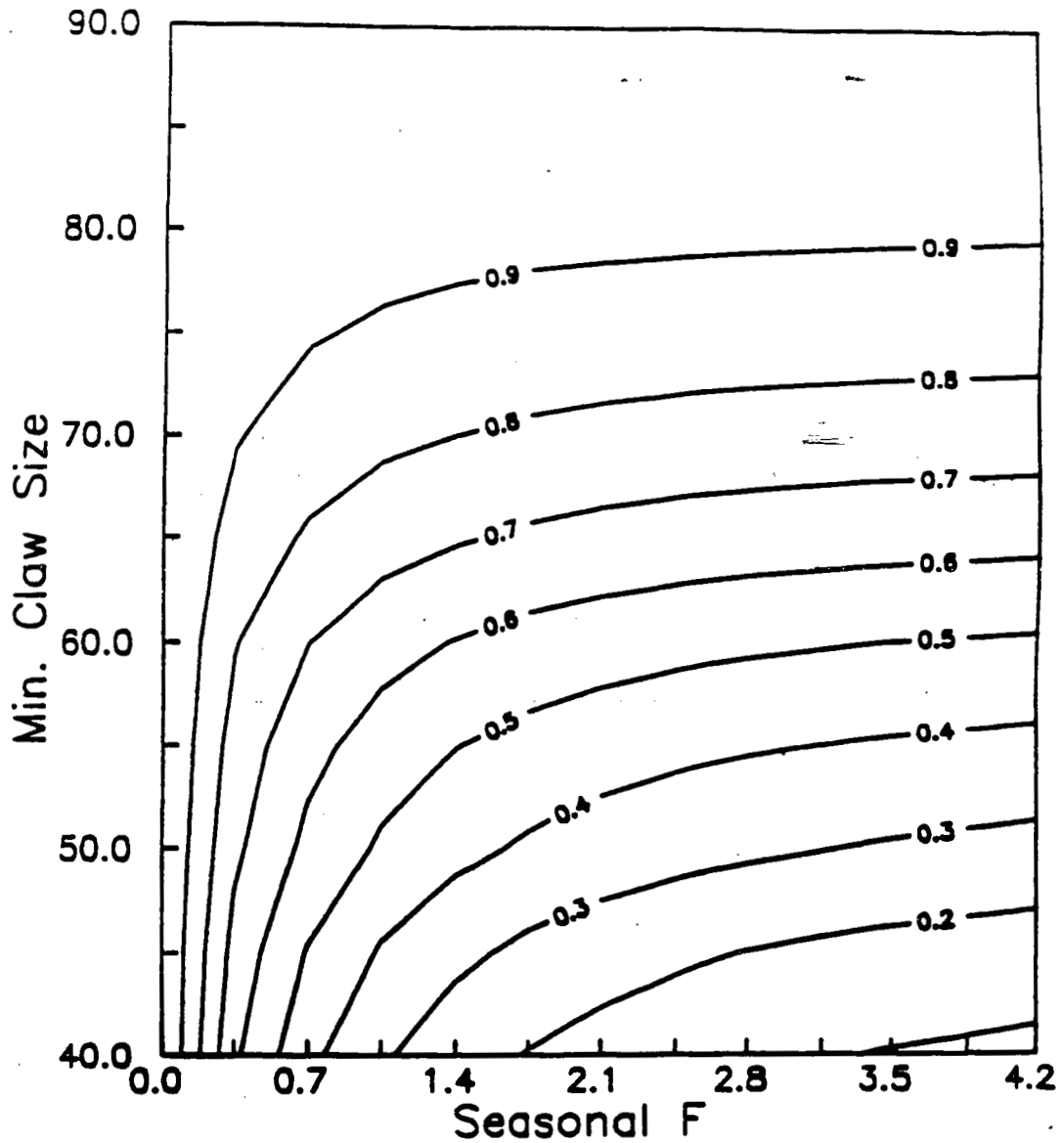
FIGURE 5: Egg production per recruit isopleths for female stone crabs under a scenario with lower natural mortality ( M=0.95 ) and full trap retention. Values are given as a fraction of those expected in an unexploited stock.
