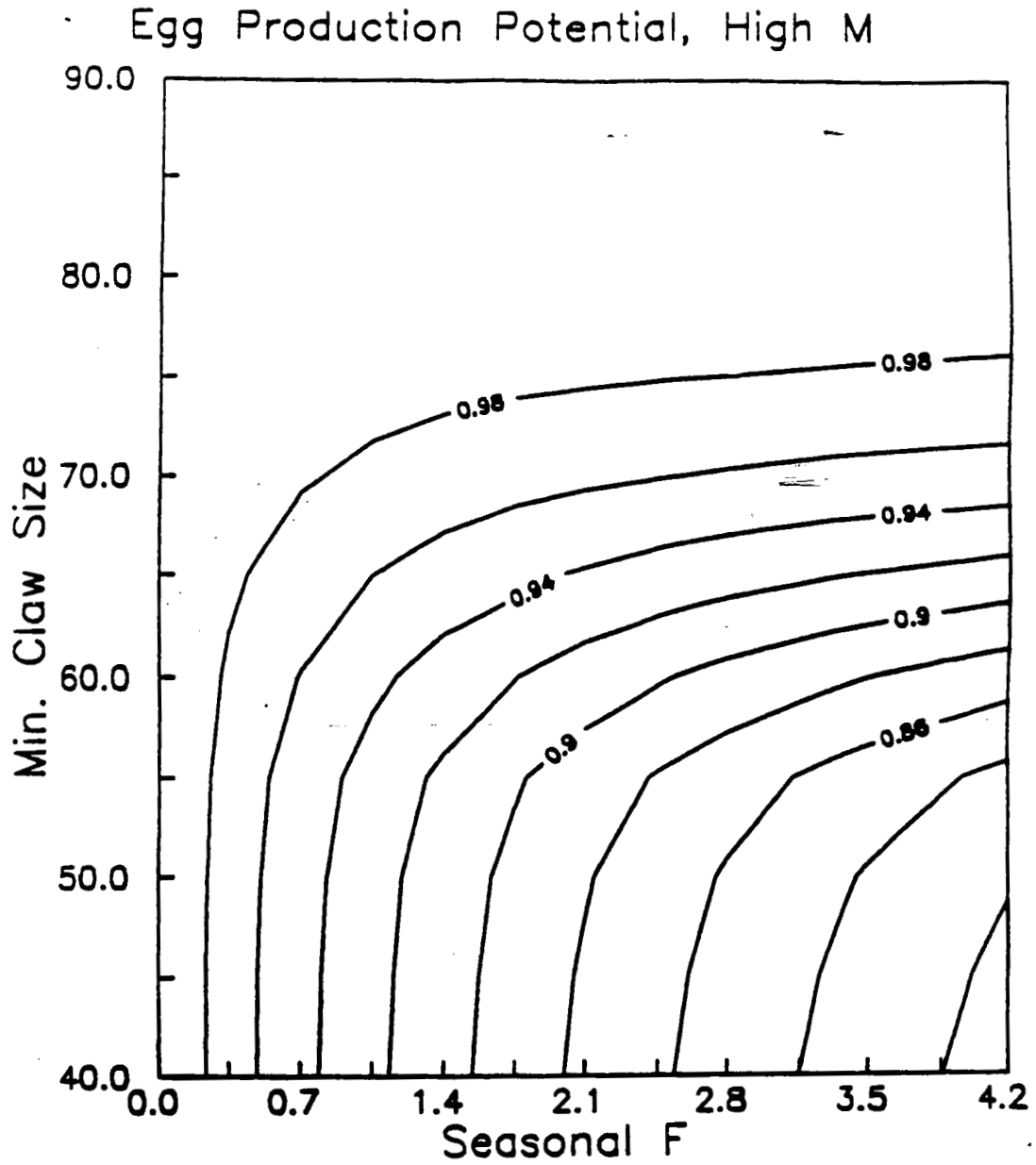
FIGURE 4: Egg production per recruit isopleths for female stone crabs under a scenario with high natural mortality ( M=1.9 ) and trap selectivity. Values are given as a fraction of those expected in an unexploited stock.
