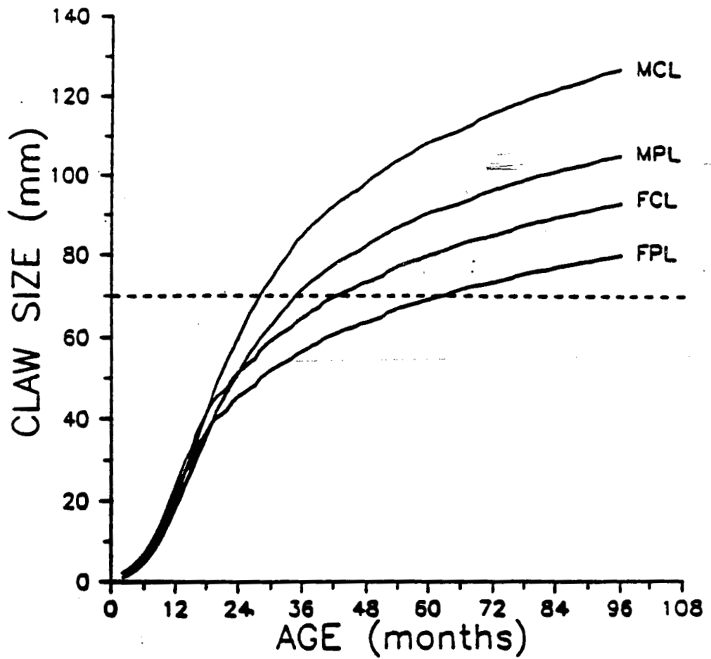
FIGURE 3: Claw growth curves for stone crabs. M = males; F = females. PL = pincer length; CL = crusher length.
